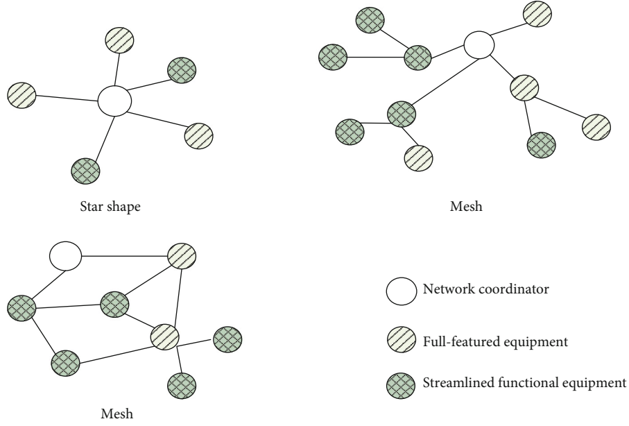
FIGURE 2: Three network topologies of the ZigBee protocol.
